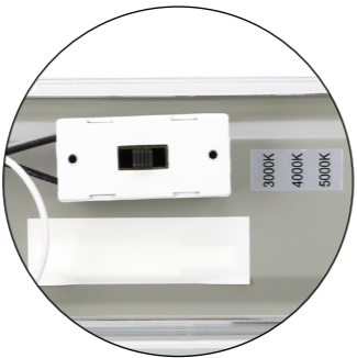
color temperature adjustment switch 3000-4000-5000K
