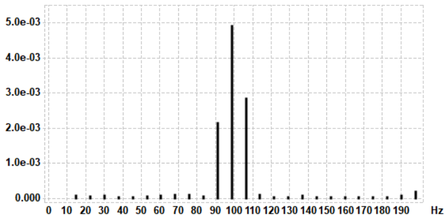
FFT chart
